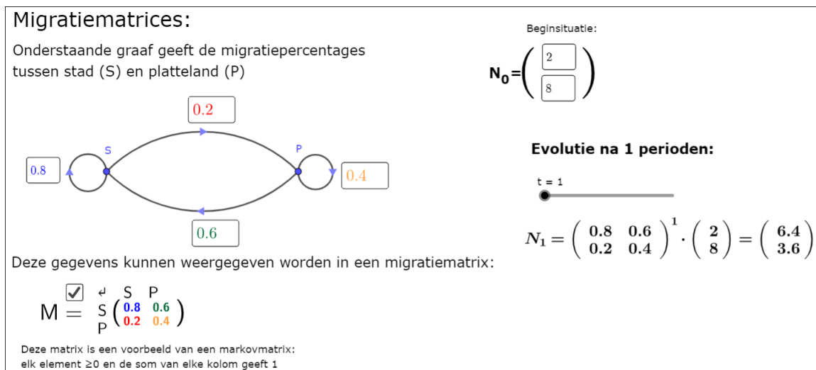
Figuur 26: https://www.geogebra.org/m/h7g2xd8b
