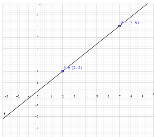
Figuur 29: https://www.geogebra.org/m/vfenrnkv
