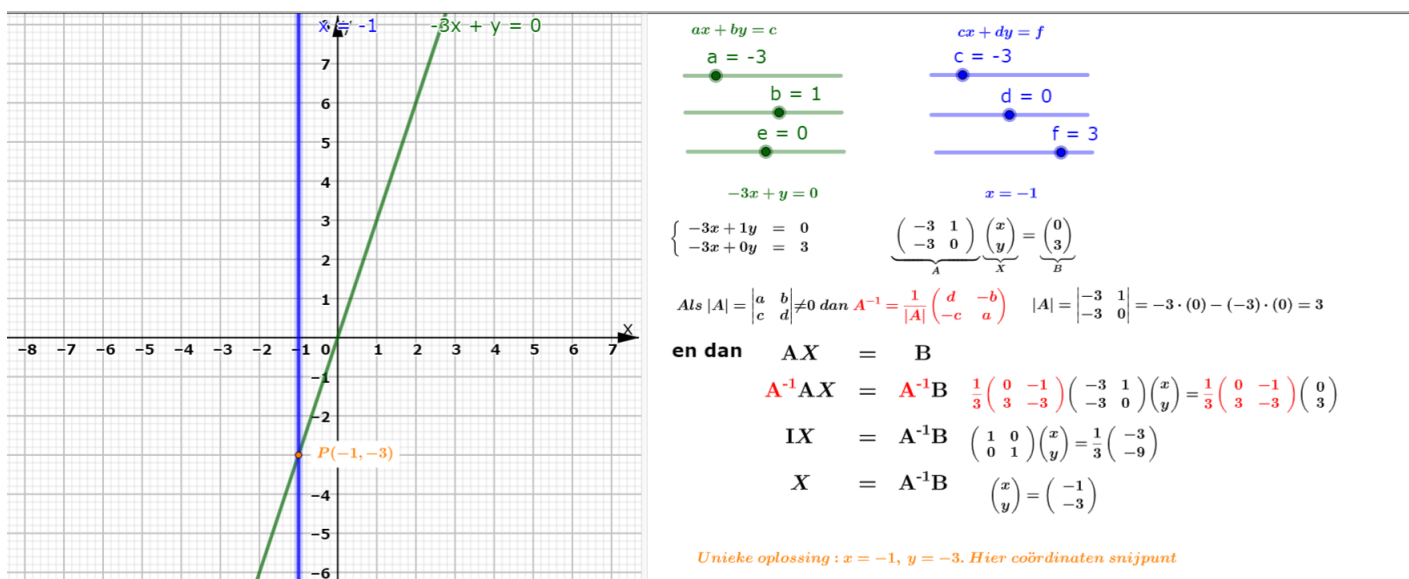
Figuur 24: https://www.geogebra.org/m/yfqw9ndn
