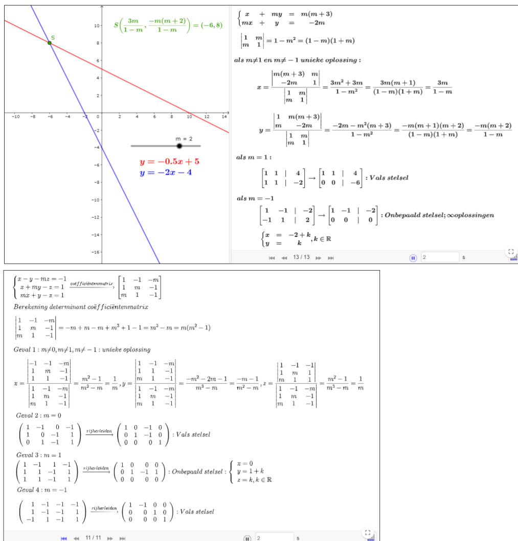
Figuur 25: https://www.geogebra.org/m/g7TcQBkv
