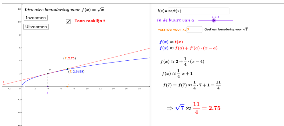
Figure 7: https://www.geogebra.org/m/NwZHM6eQ
