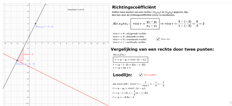
Figure 1: https://www.geogebra.org/m/V6dh2XPP
