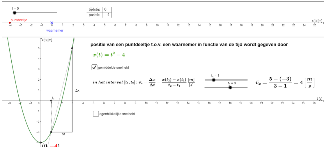
Figure 12: https://www.geogebra.org/m/nsGgY8T3
