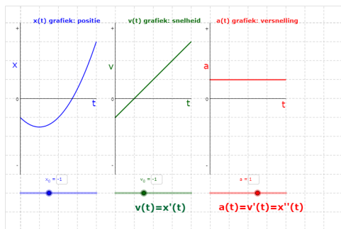
Figure 13: https://www.geogebra.org/m/nsGgY8T3
